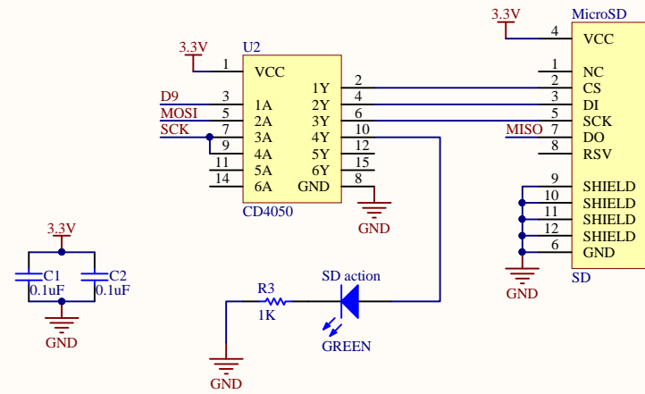
Level buffer
